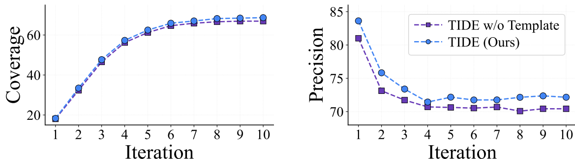
FIGURE 6 Per-iteration retrieval coverage (left) and precision (right) on the Workspace setting with GPT.
