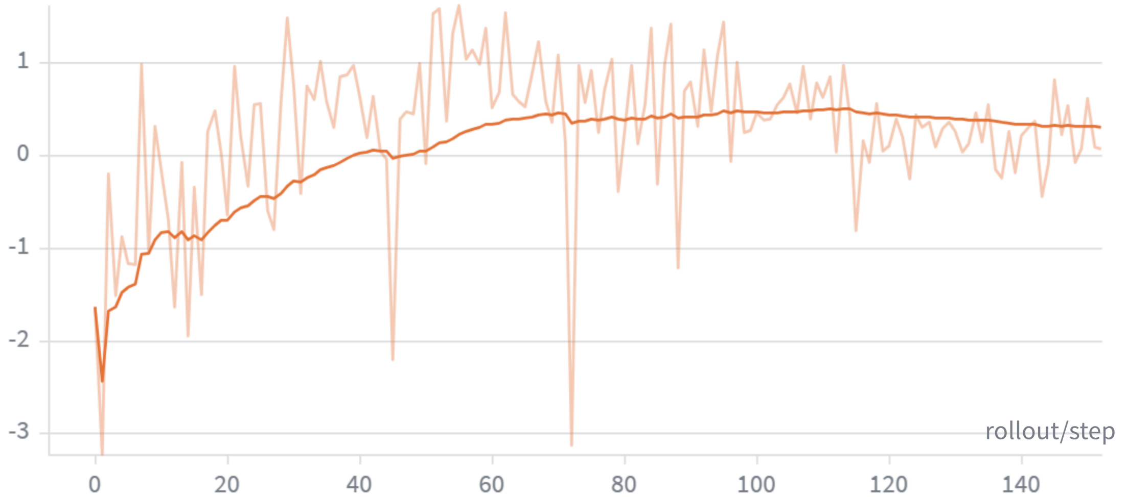
rollout/raw_reward
