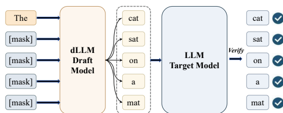
FIGURE 1 Diffusion-based speculative decoding with a dLLM draft model. The dLLM proposes a block of tokens in parallel, while the target LLM verifies the block and accepts the longest consistent prefix.
