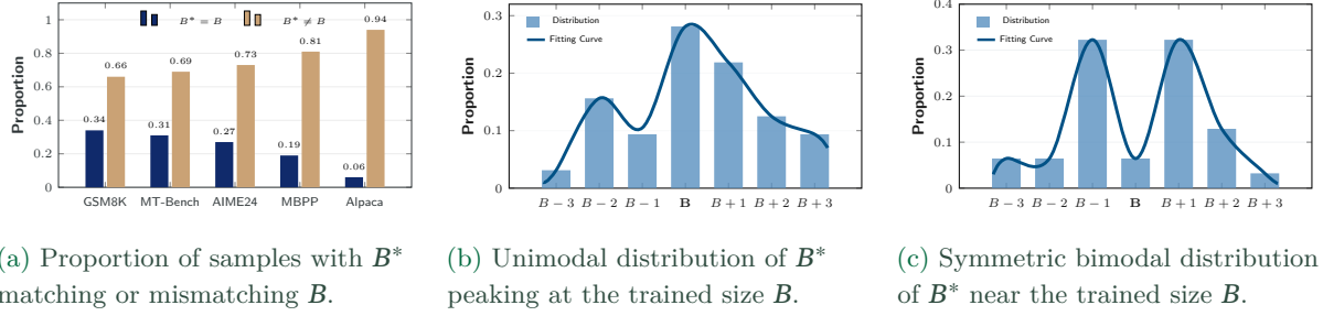
FIGURE 3 Analysis of optimal block size B^* . (a) Matching and mismatching proportions across datasets. (b-c) Distribution patterns demonstrating strong locality, where the range [B - 3, B + 3] covers the optimal size for nearly all samples.
