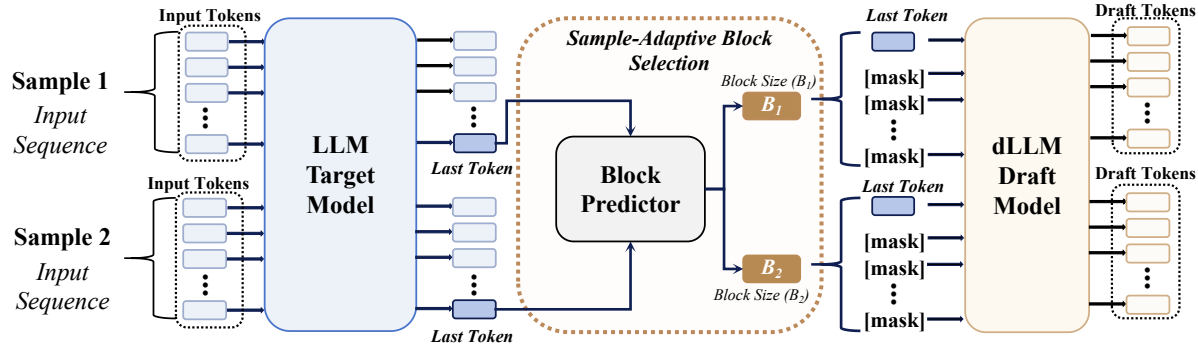
FIGURE 4 Overview of the BlockPilot inference pipeline. Given an input sequence, the target LLM performs prefilling and produces the predictive distribution of the last token, which serves as a compact representation of the decoding state. This distribution is then fed into a lightweight block size predictor to determine an instance-specific block size. Based on the predicted block size, the diffusion-based draft model generates a block of draft tokens in parallel.
