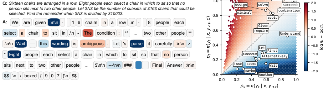
Figure 2: Per-token signal u_t = t_t - s_t on Qwen3-4B-IT-2507 at AIME-25. (a) Single-rollout trace. (b) (\pi_S, \pi_T) heatmap. Blue marks deliberation tokens ( u_t \ll 0 ); red marks shortcut tokens ( u_t \gg 0 ). plays two roles: the student \pi_S(\cdot | x, y_{<t}) := \pi_\theta(\cdot | x, y_{<t}) generates the rollout, while the teacher \pi_T(\cdot | x, y_{<t}) := \pi_\theta(\cdot | x, c, y_{<t}) scores it under richer conditioning (we suppress c from the teacher’s left-hand-side conditioning as a notational shorthand, since c is fixed throughout each training step). With \text{sg}[\cdot] denoting stop-gradient, the standard self-distillation loss is the per-token KL,
