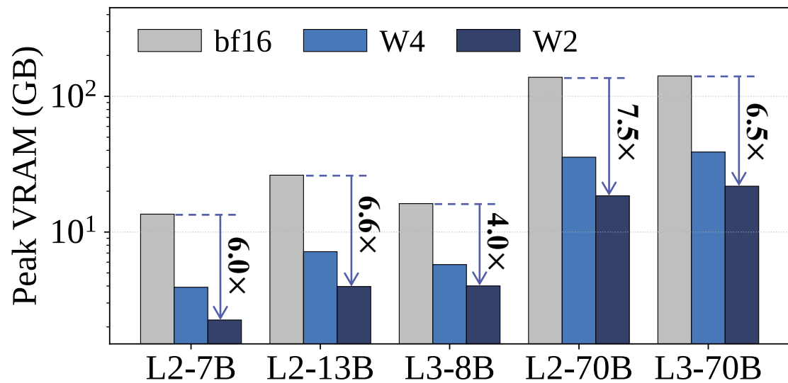
(a) Peak inference VRAM (GB) across precisions
