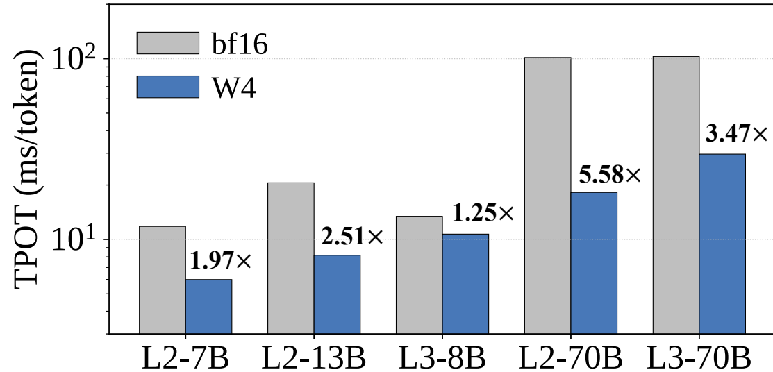
(b) Decoding latency (TPOT, ms/token)
