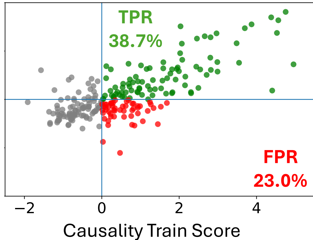
(b) Causal Regions Discovery
