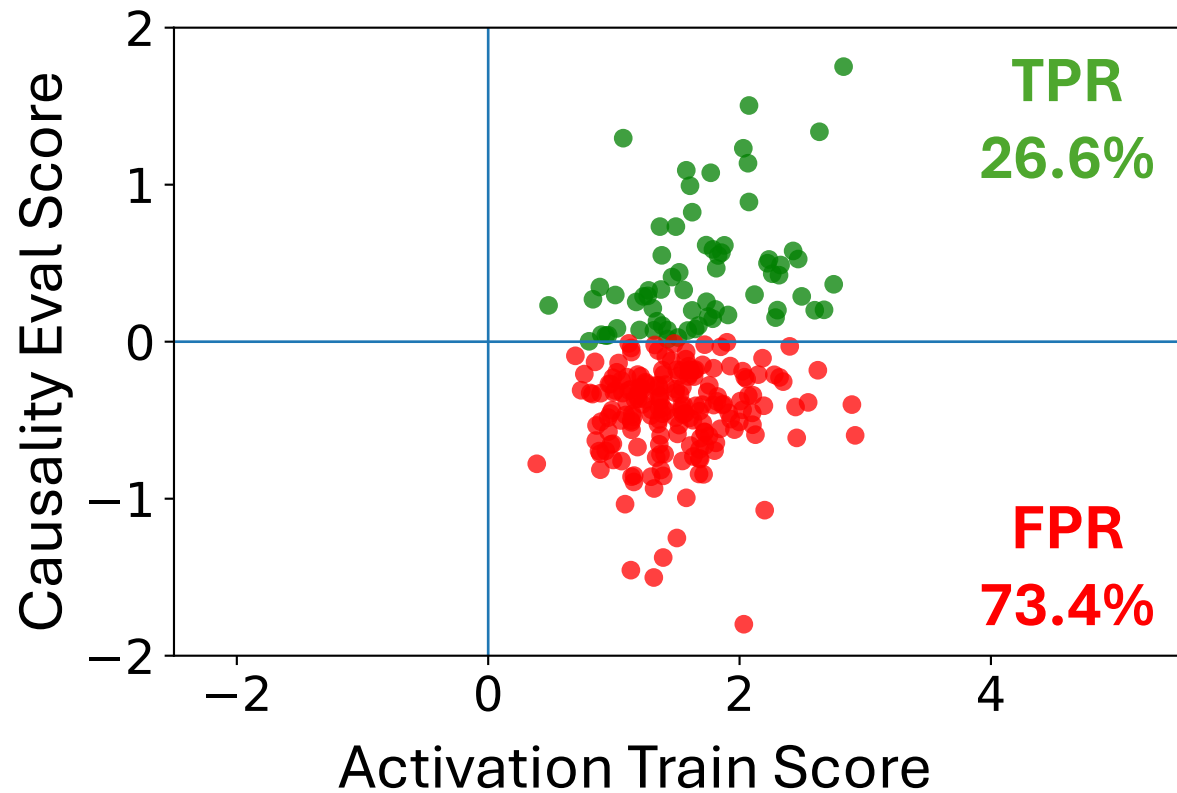
(a) Non-Causal Regions Discovery
