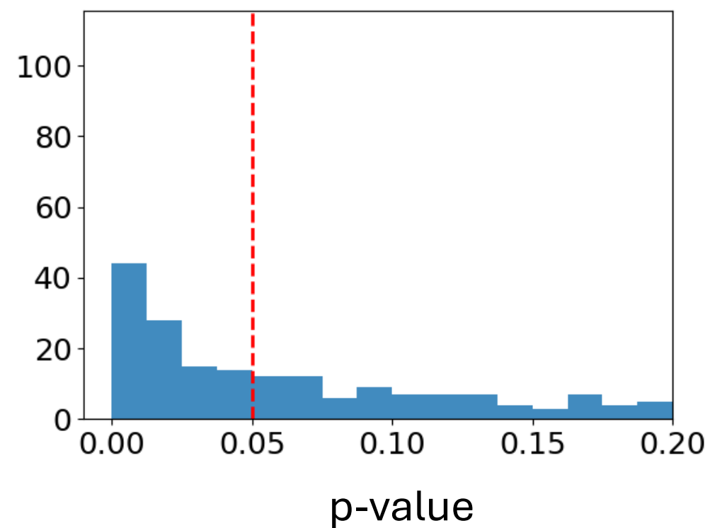
Counterfactual Causality
