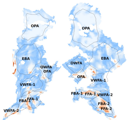
Causal Score
