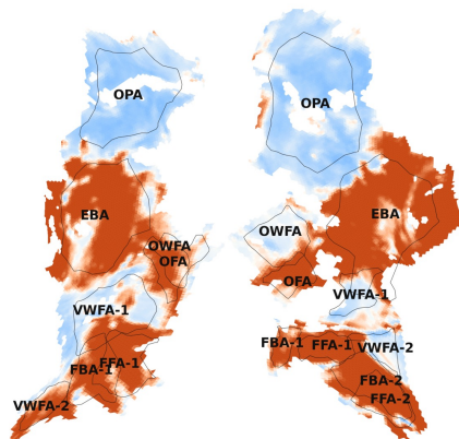
Activation Score
