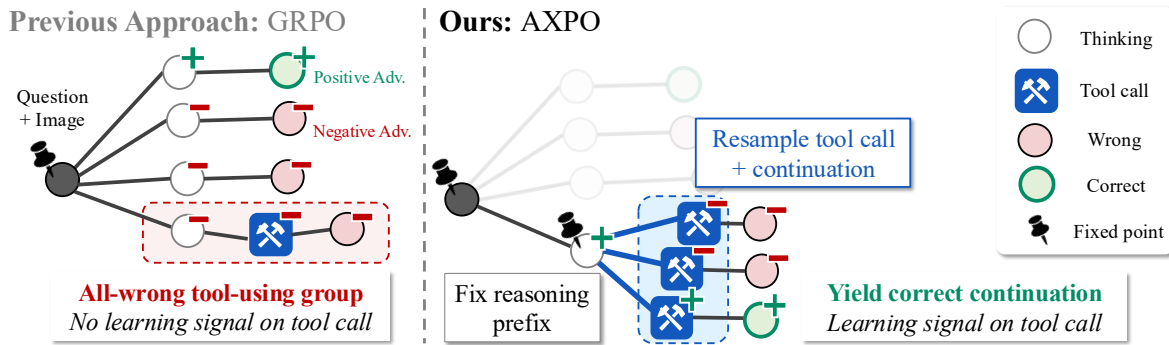
FIGURE2 Concept. AXPO concentrates exploration on the tool call for agentic reasoning. Left: under GRPO, tool-using rollouts are scarce and often fail, leaving no positive learning signal at the tool call where it is most needed. Right: AXPO fixes the thinking prefix from the failed rollout and resamples the tool call and its continuation, recovering a correct rollout and producing a positive learning signal on the tool call.
