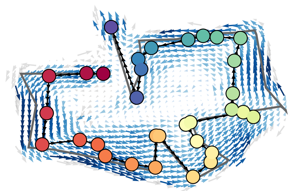
C Average delayed recall events
