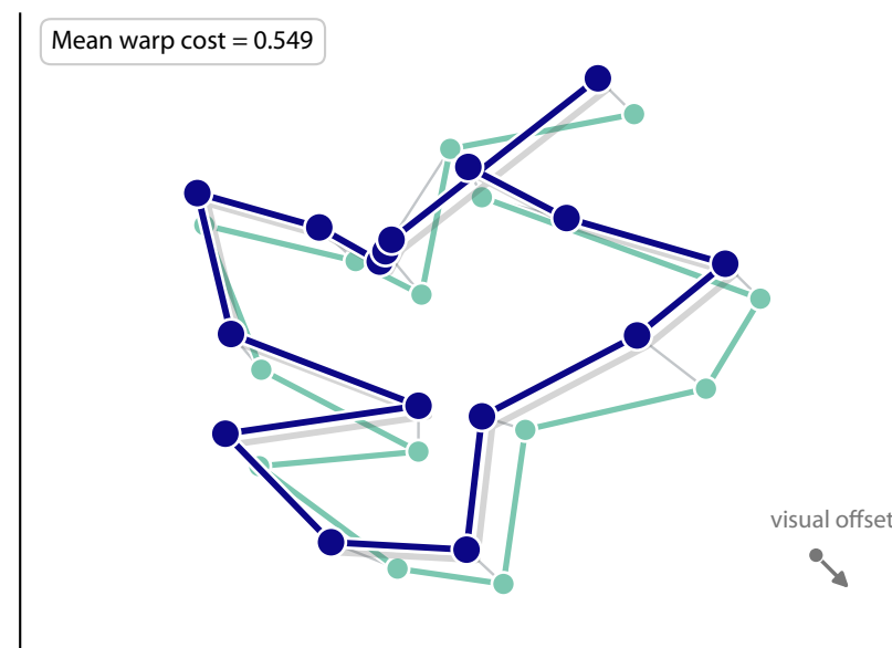
A P2 delayed recall ↔ P2 immediate recall
