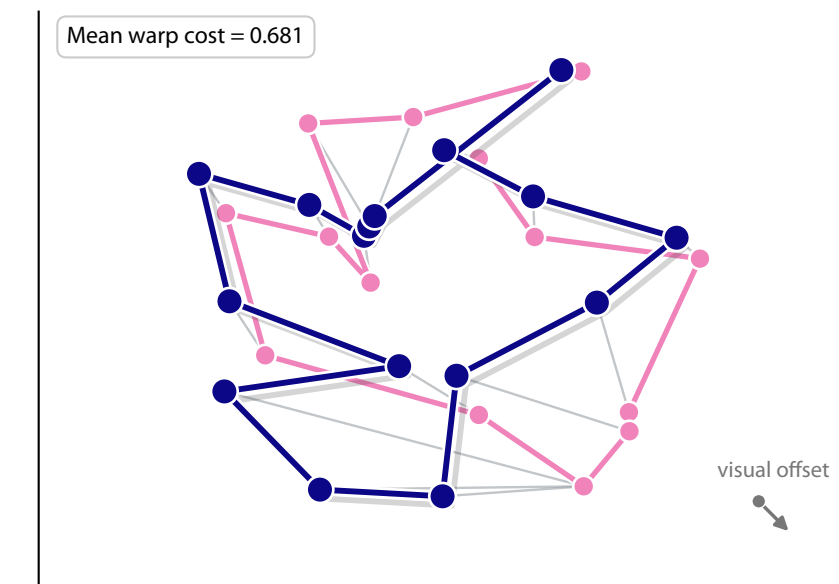
B P2 delayed recall ↔ P10 immediate recall
