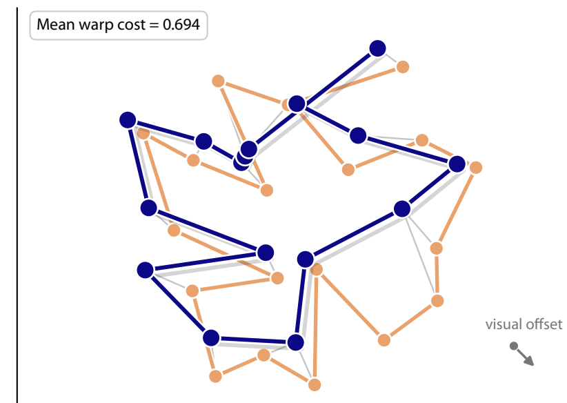
C P2 delayed recall ↔ episode
