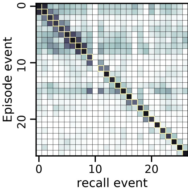
Average Atlanta episode 2-recall events correlation matrix
