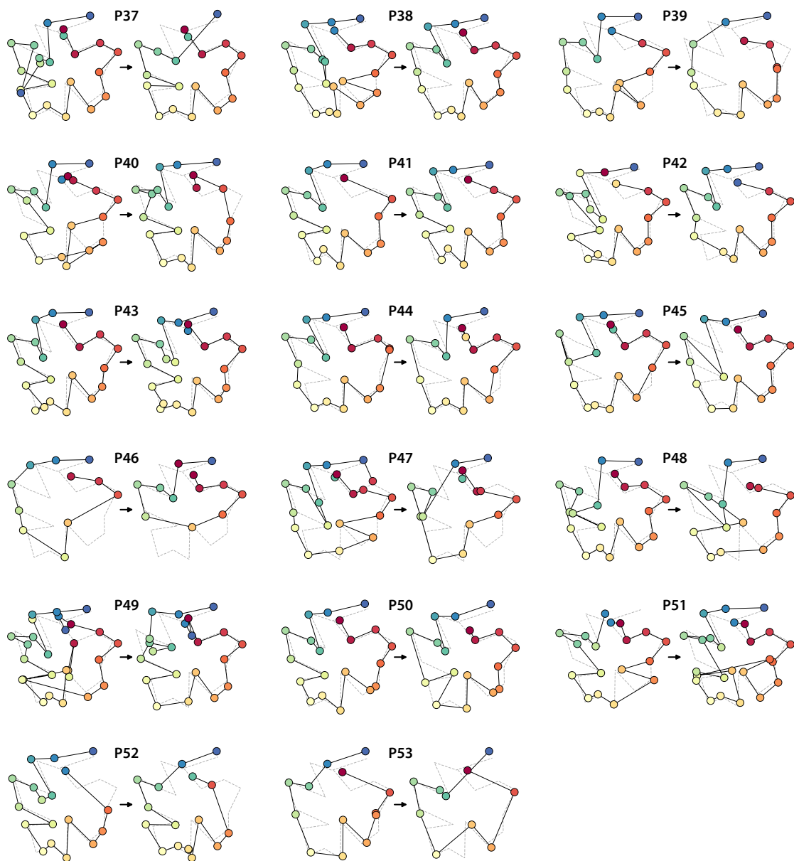
Supplementary Figure 3: 2D projections all participants' recall trajectories. Each pair of trajectories (left: immediate recall; right: delayed recall) is in the same format as those displayed in Figure 4.
