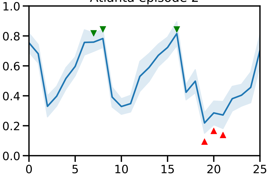
Atlanta episode 2
