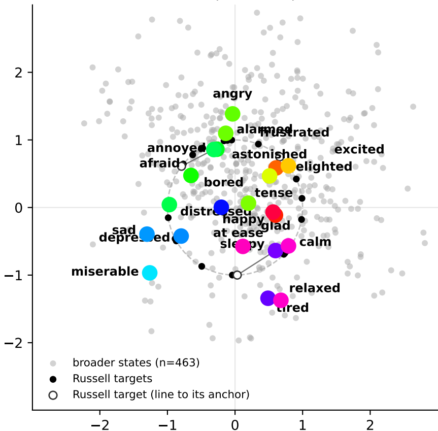
all-states PC6+PC9 | layer 26 | disparity 0.28
