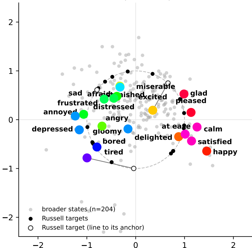
all-states PC4+PC7 | layer 16 | disparity 0.43
