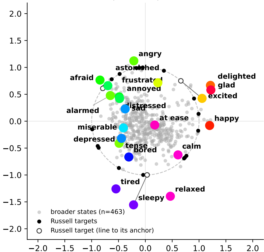
PC1+PC2 | layer 21 | disparity 0.33
