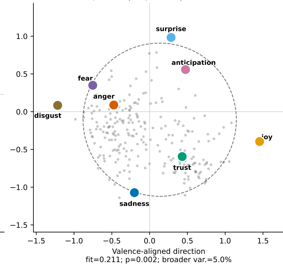
Spanish | layer 31 | PC1+PC2
