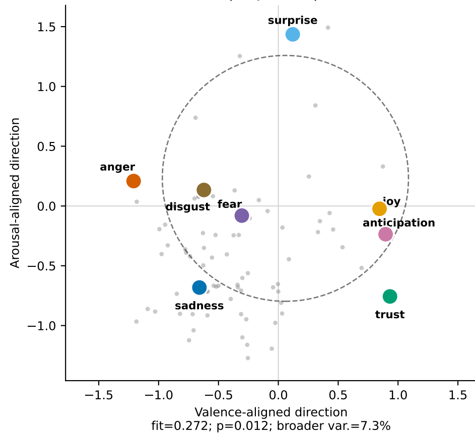
Romanian | layer 18 | PC1+PC2
