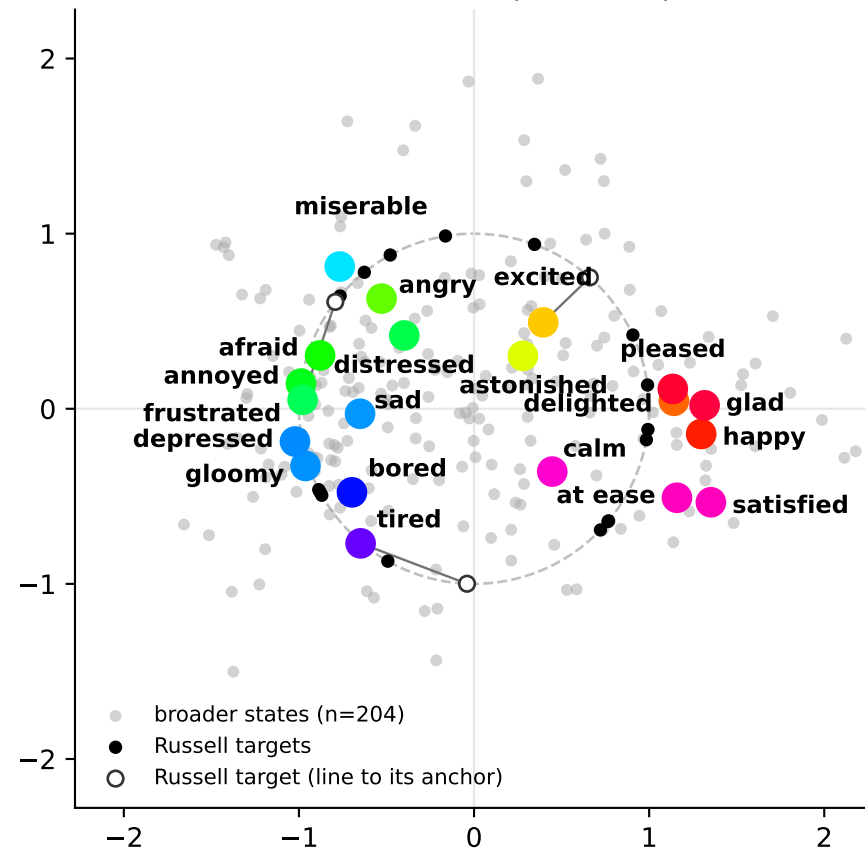
Persian — all-states PC3+PC9 | layer 12 | disparity 0.26
