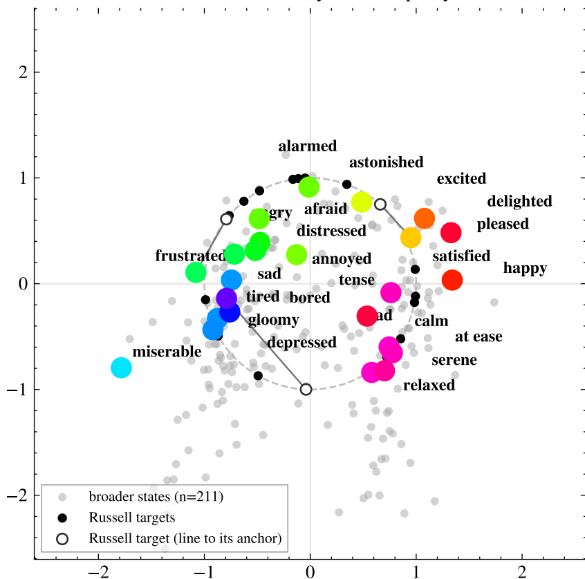
all-states PC1+PC2 | layer 20 | disparity 0.24
