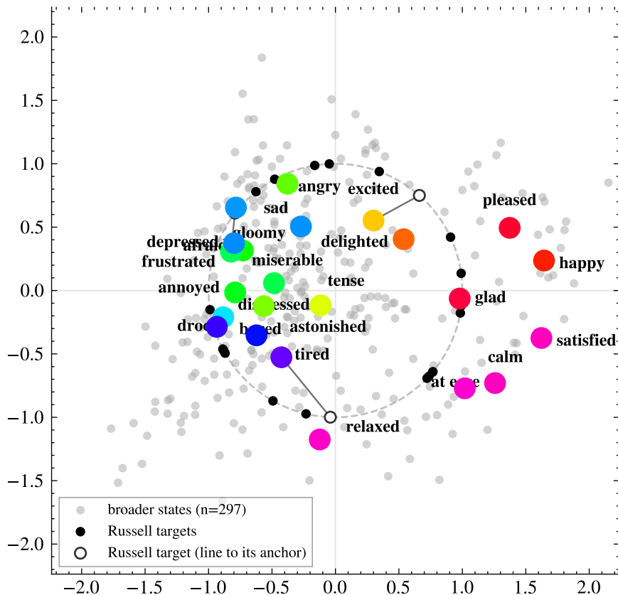
all-states PC2+PC5 | layer 20 | disparity 0.48
