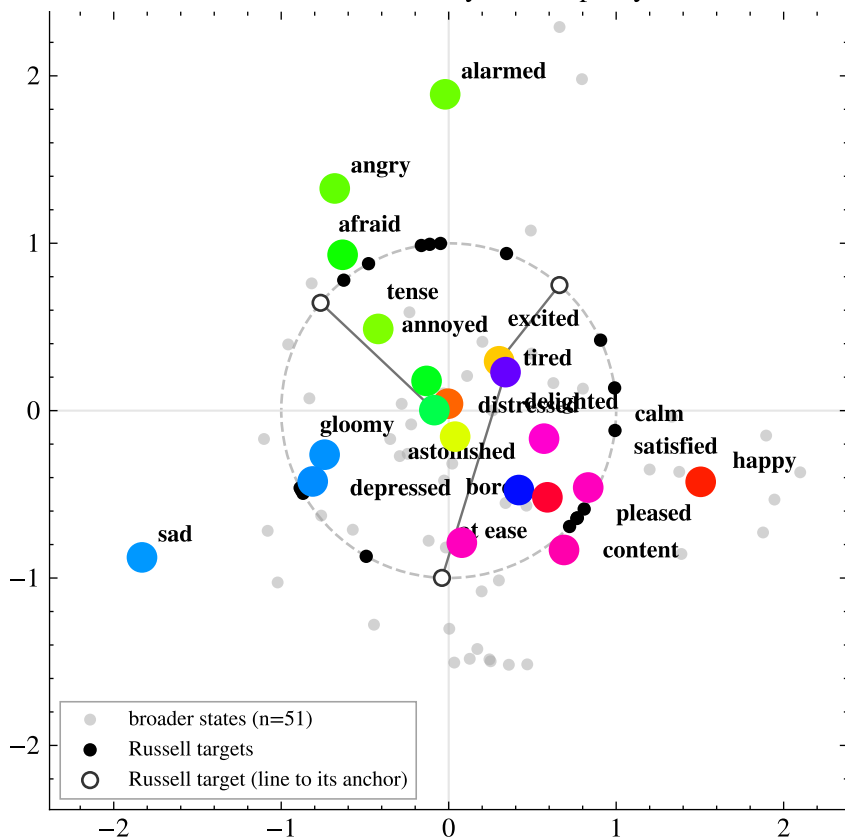
all-states PC6+PC8 | layer 9 | disparity 0.48
