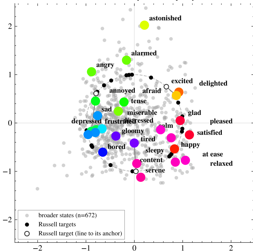
all-states PC2+PC3 | layer 17 | disparity 0.30
