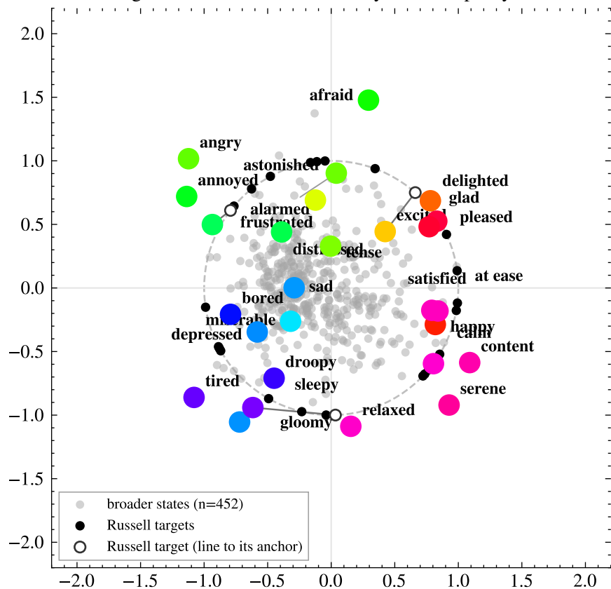
English: searched PC2+PC3 | layer 10 | disparity 0.31
