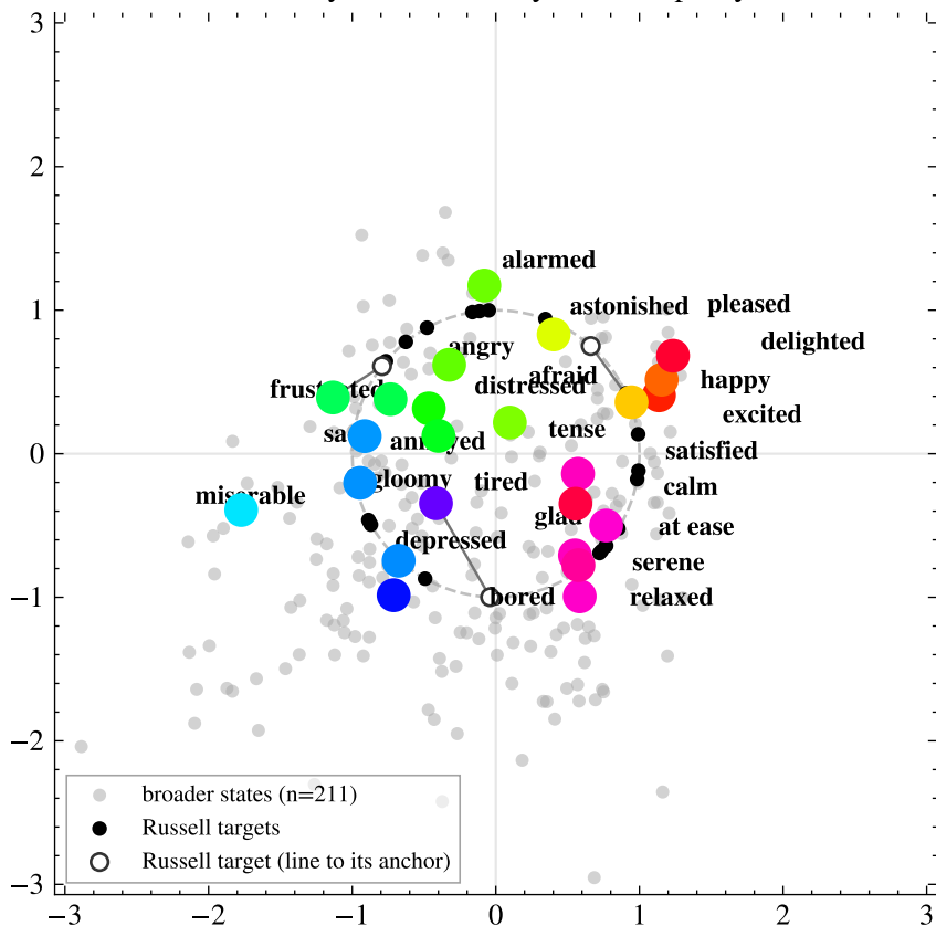
broader-only PC1+PC3 | layer 17 | disparity 0.22
