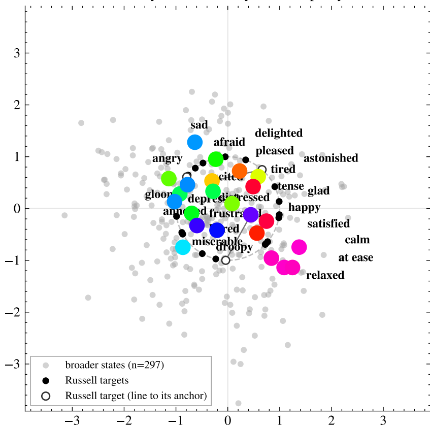
broader-only PC5+PC8 | layer 20 | disparity 0.52
