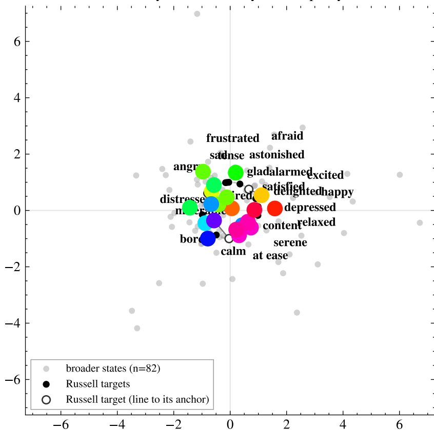
broader-only PC3+PC9 | layer 8 | disparity 0.39
