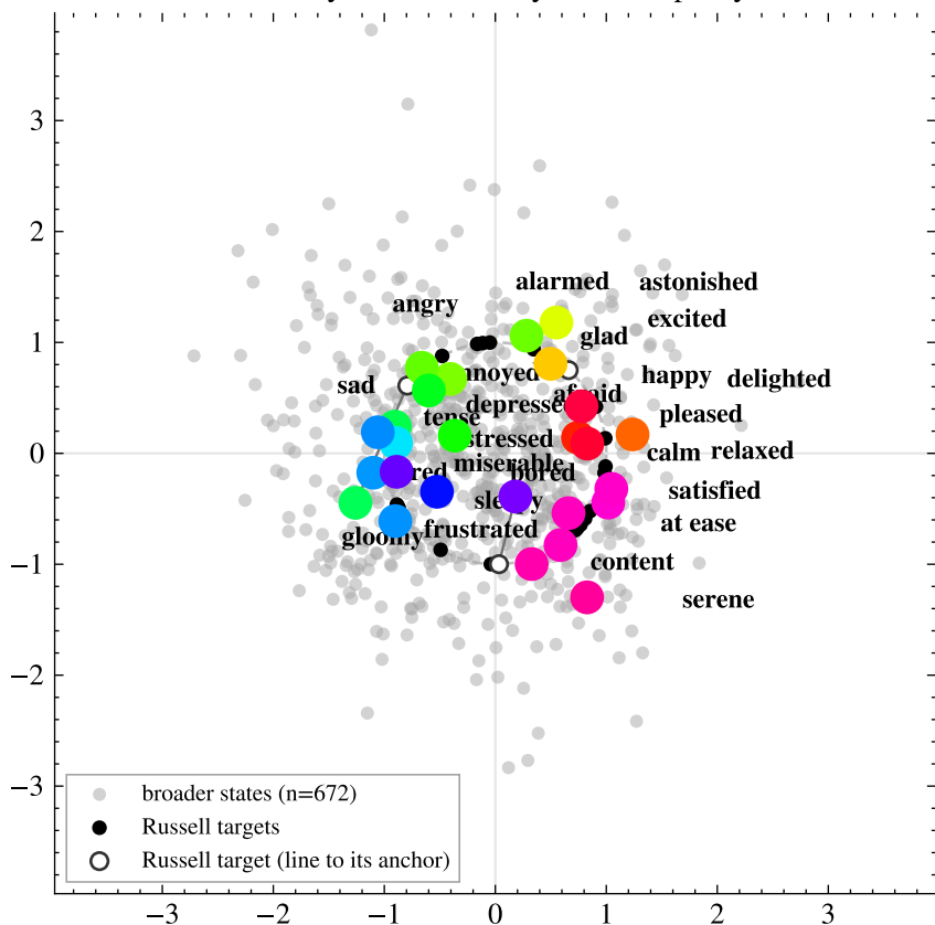
broader-only PC4+PC5 | layer 36 | disparity 0.27
