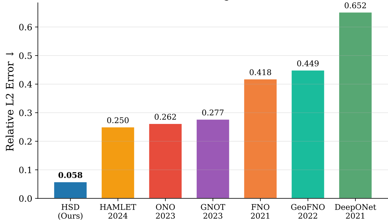
Torus Helmholtz (genus-1, 0 \rightarrow 1)
