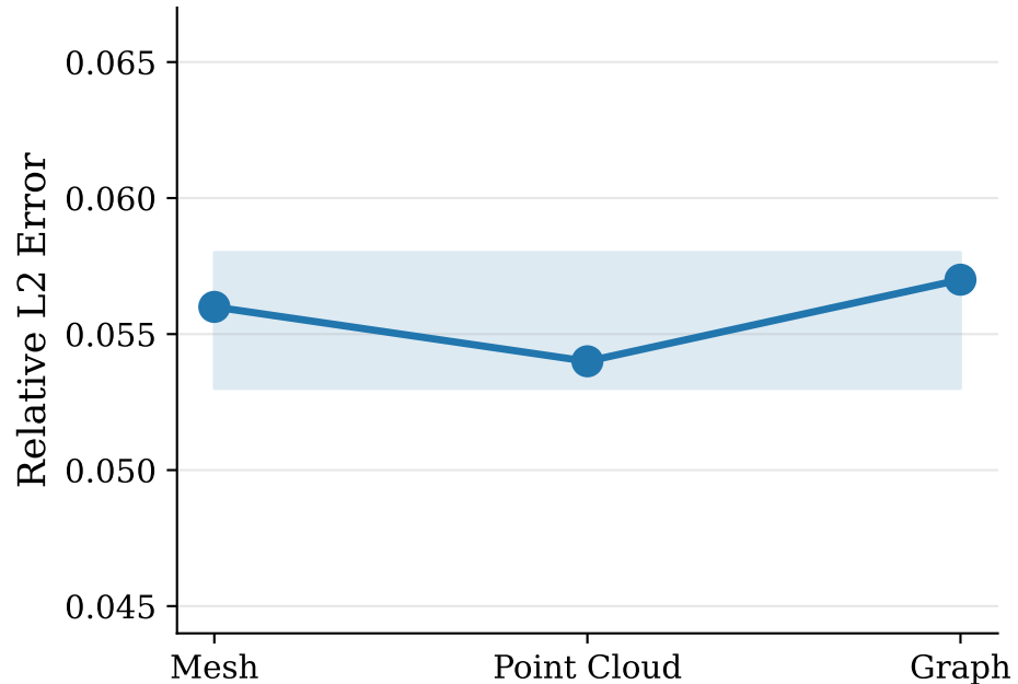
Torus (genus-1) spread = 0.0030
