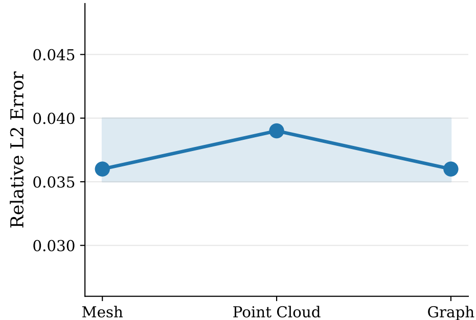
Ellipsoid (genus-0) spread = 0.0030
