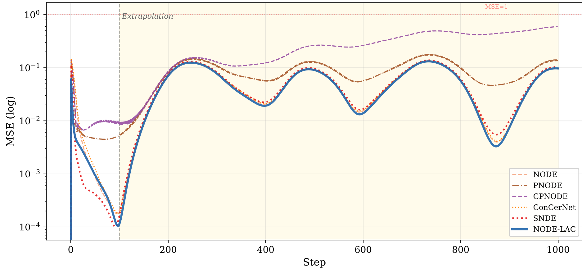
FitzHugh-Nagumo — Error Evolution (1000 steps)
