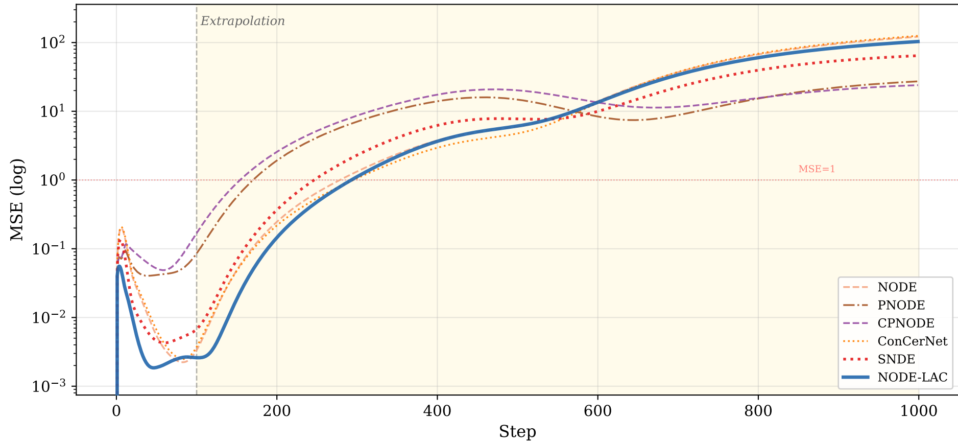
Lotka-Volterra — Error Evolution (1000 steps)
