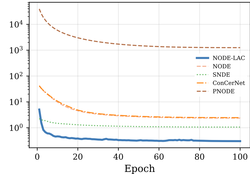
Shallow Water
