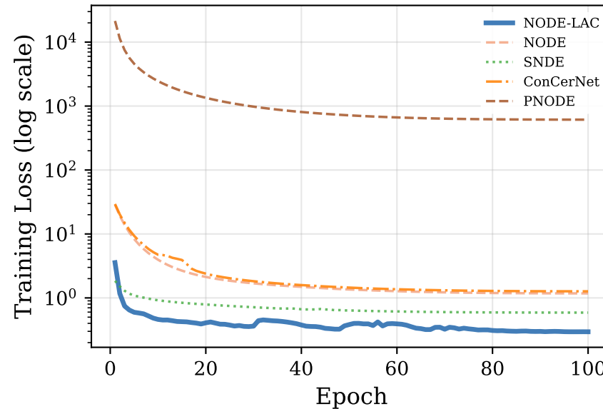
FitzHugh-Nagumo
