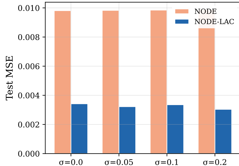
FitzHugh-Nagumo
