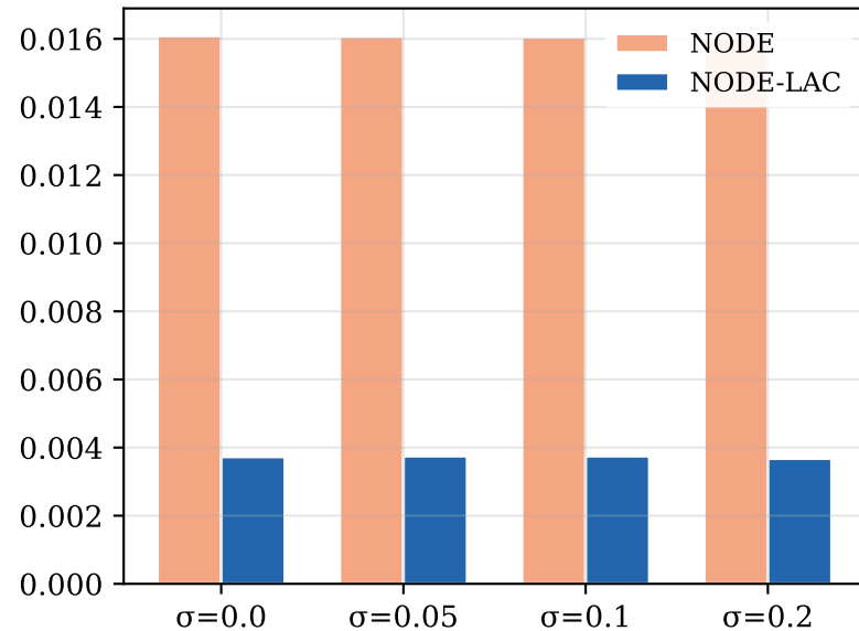
Shallow Water
