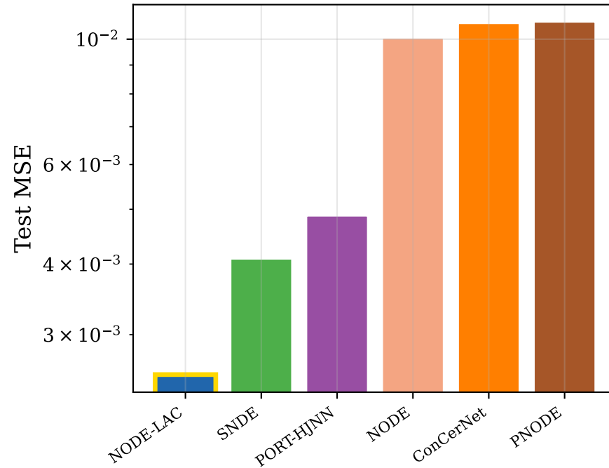
FitzHugh-Nagumo
