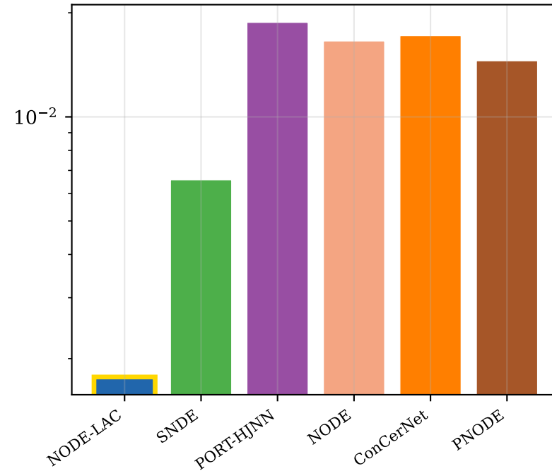
Shallow Water
