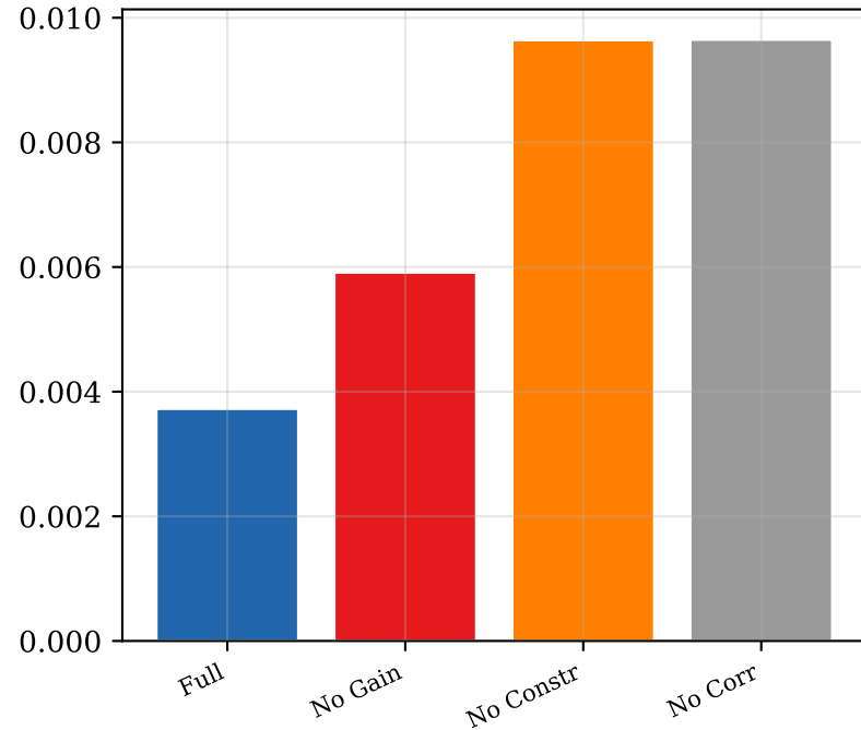
Shallow Water
