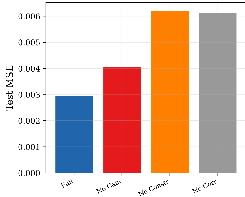
FitzHugh-Nagumo
