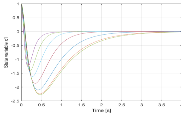
Figure 4.1: Approximate and optimal state variables x_1(t)
