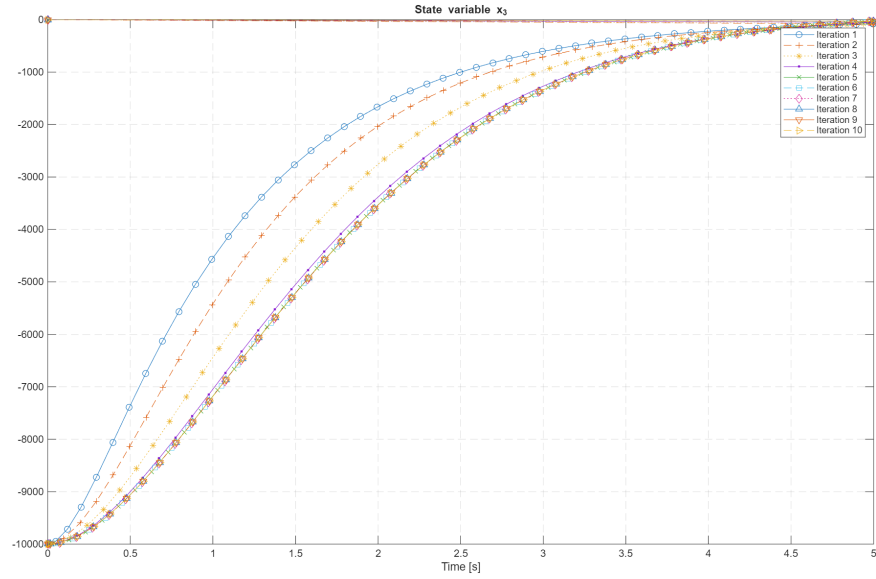
Figure 4.11: Approximate and optimal state trajectory x_3(t)
