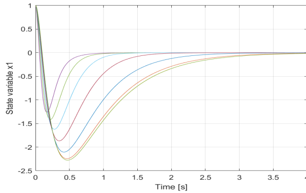
Figure 4.1: Approximate and optimal state variables x_1(t)
