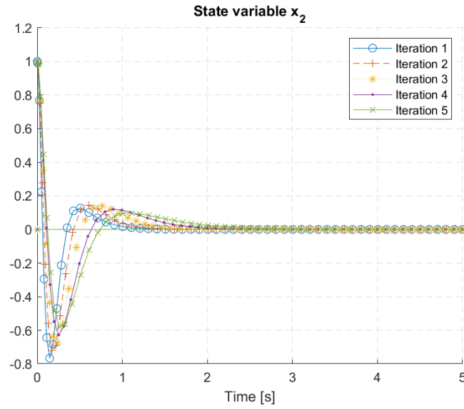
Figure 4.9: Approximate and optimal x_2(t) state variable
