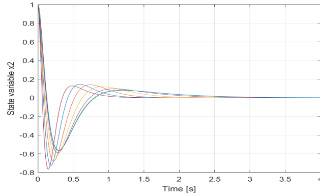
Figure 4.2: Approximate and optimal state variables x_2(t)
