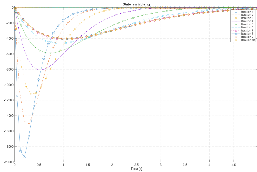
Figure 4.12: Approximate and optimal state trajectory x_4(t)
