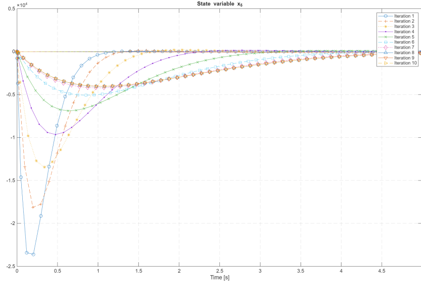
Figure 4.13: Approximate and optimal state trajectory x_5(t)
