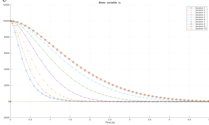
Figure 4.9: Approximate and optimal state trajectory x_1(t)
