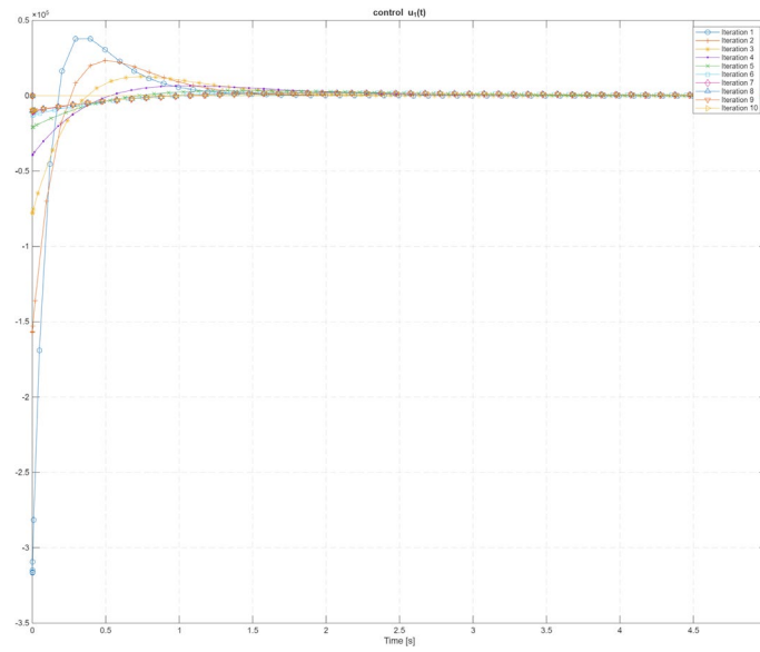
Figure 4.15: Approximate and optimal control u_1(t)
