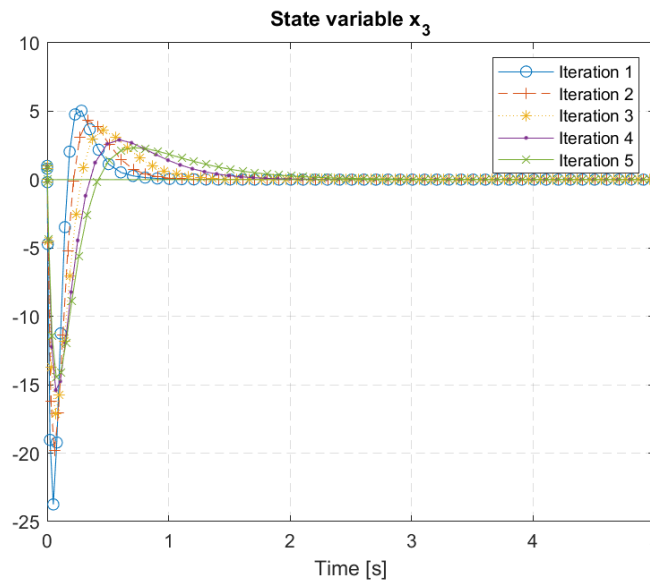
Figure 4.10: Approximate and optimal x_3(t) state variable
