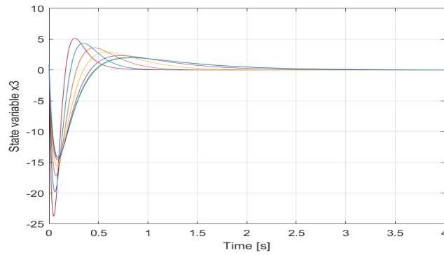
Figure 4.3: Approximate and optimal state variables x_3(t)
