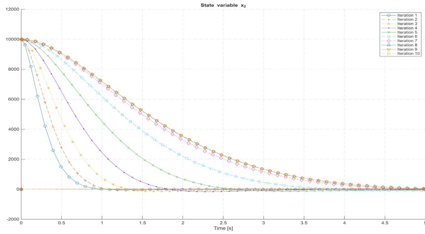
Figure 4.10: Approximate and optimal state trajectory x_2(t)
