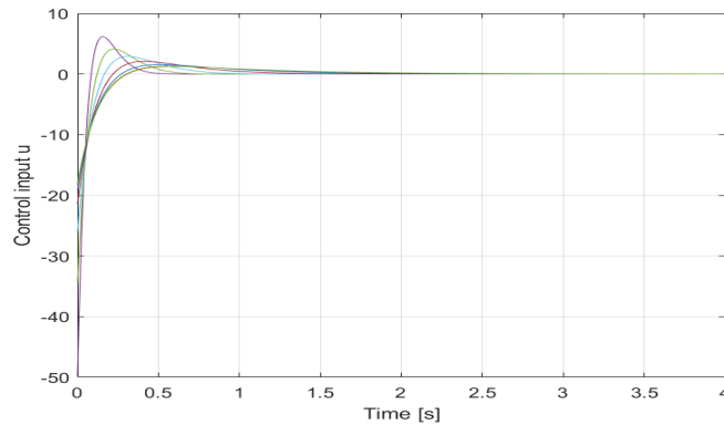
Figure 4.5: Approximate and optimal feedback controls u(x(t))
