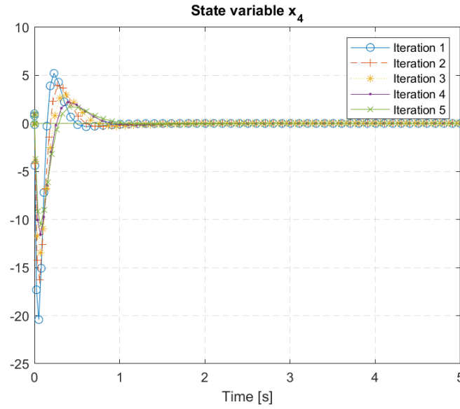
Figure 4.11: Approximate and optimal x_4(t) state variable
