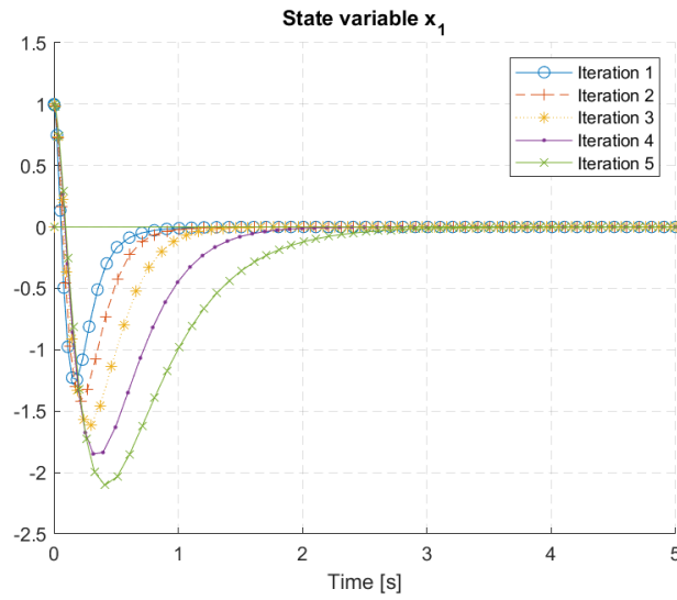
Figure 4.8: Approximate and optimal x_1(t) state variable
