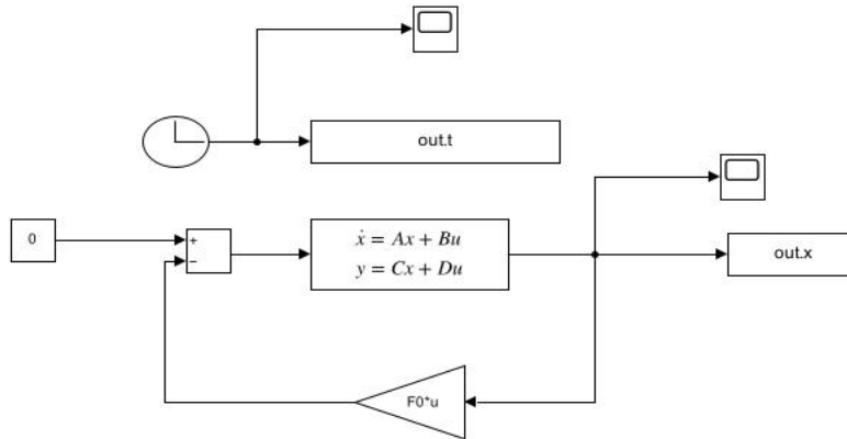
Figure 4.7: Pendulum Simulink model
