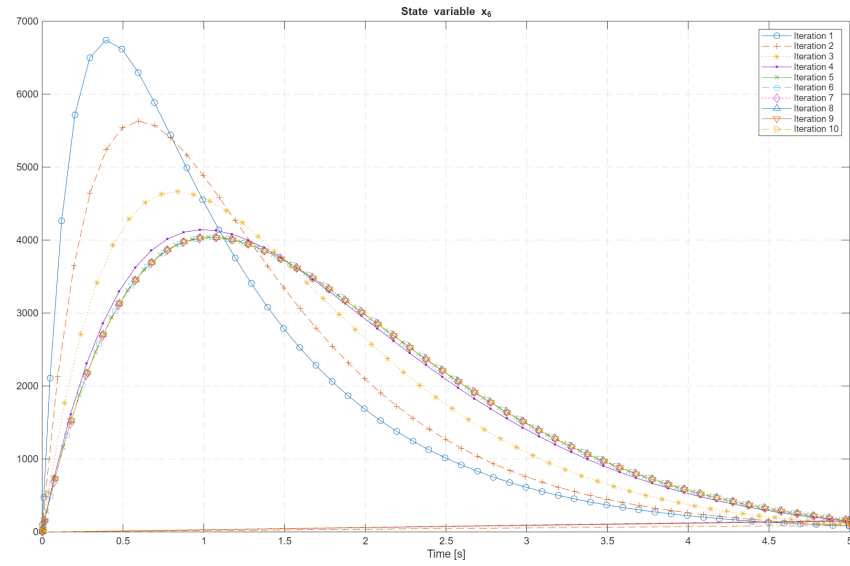
Figure 4.14: Approximate and optimal state trajectory x_6(t)
