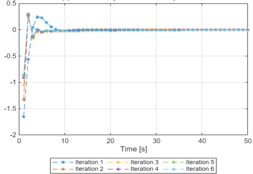
Iteration-wise Approximate System State Trajectories for Variable x_3
