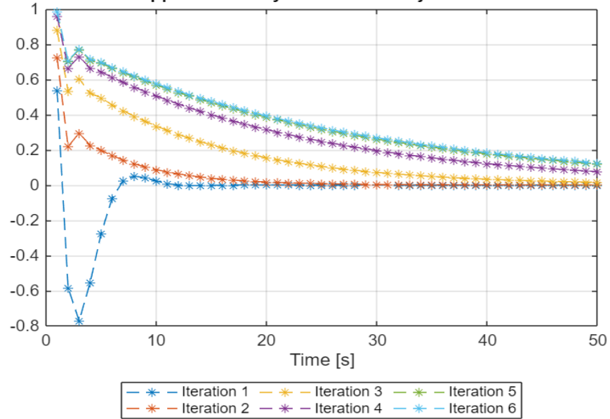
Iteration-wise Approximate System State Trajectories for Variable x_4
