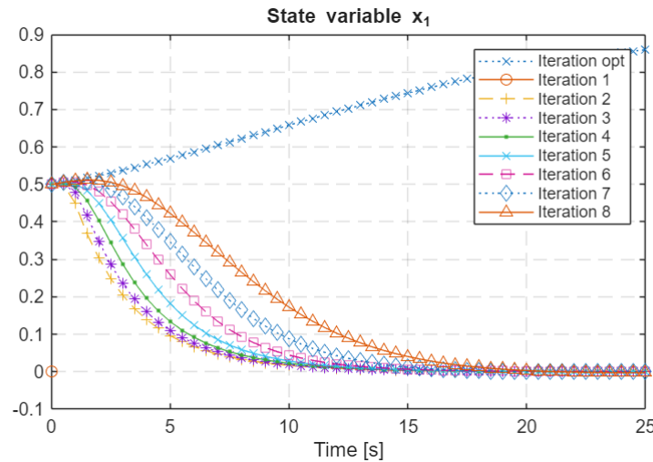
Figure 3.9: Approximate and optimal state trajectories x_1(t)
