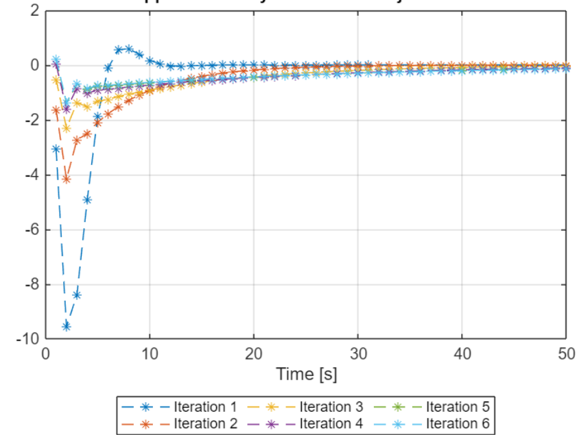
Iteration-wise Approximate System State Trajectories for Variable x_2
