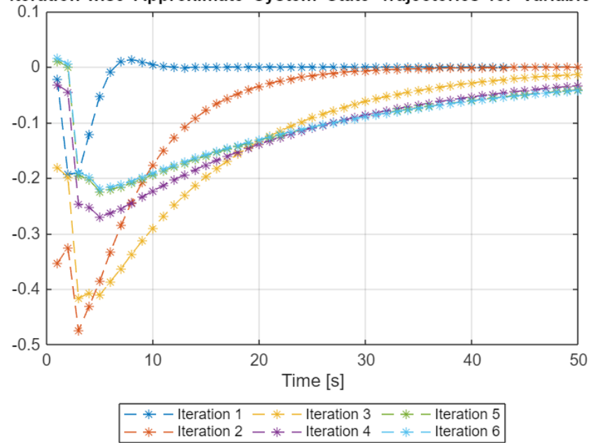
Iteration-wise Approximate System State Trajectories for Variable x_1
