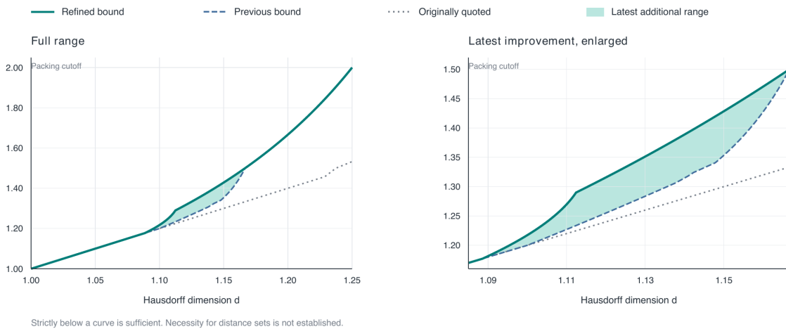
Figure 1: The refined sufficient curve, the preceding unforced curve, and the originally quoted curve. The second panel isolates the latest improvement. Values strictly below a curve are covered. No curve is asserted to be necessary.
