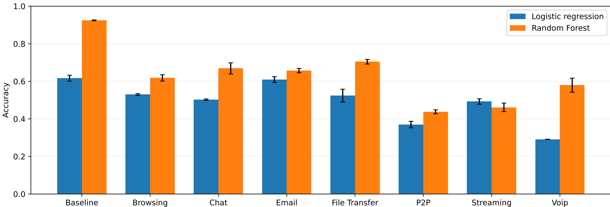
VPN classification: random baseline and category-held-out evaluation Five runs; bars = mean, error bars = sample standard deviation
