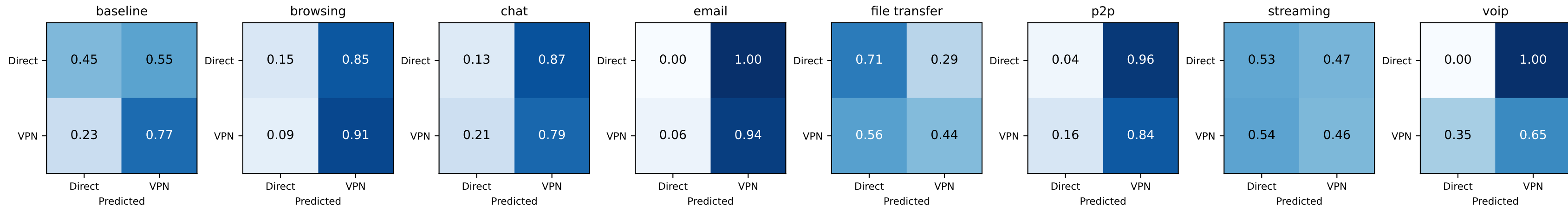
Mean row-normalized confusion matrices across five runs
