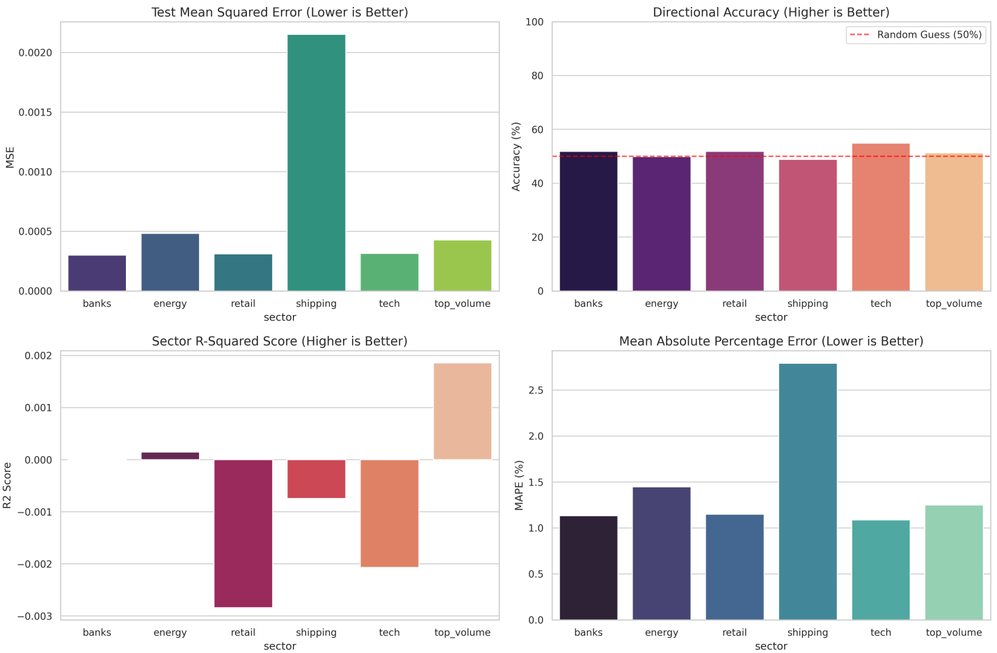
Cross-Sector Model Performance Comparison
