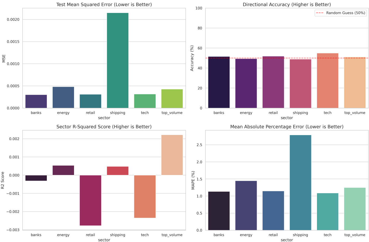
Cross-Sector Model Performance Comparison
