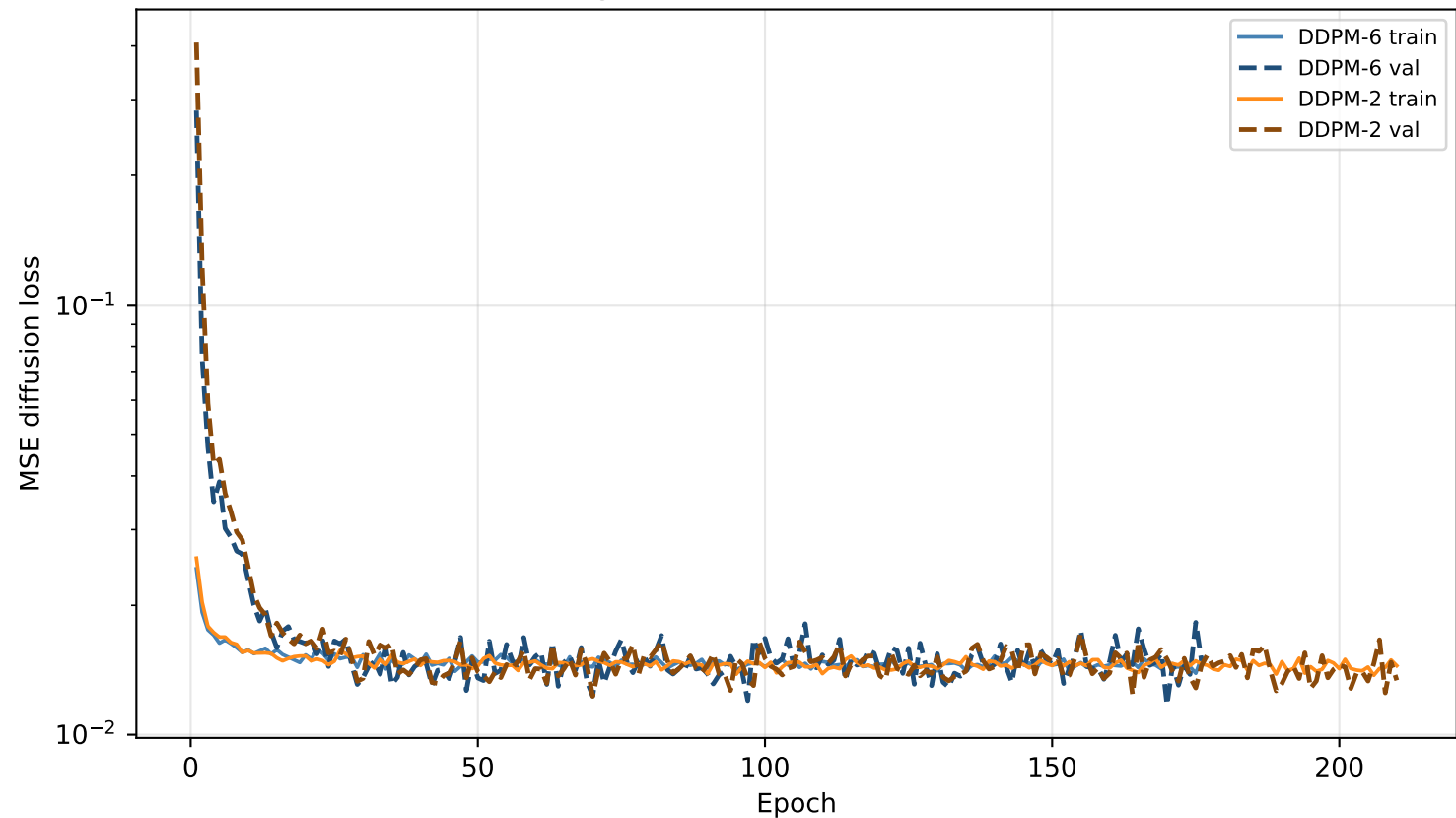
Training / validation curves (combined)
