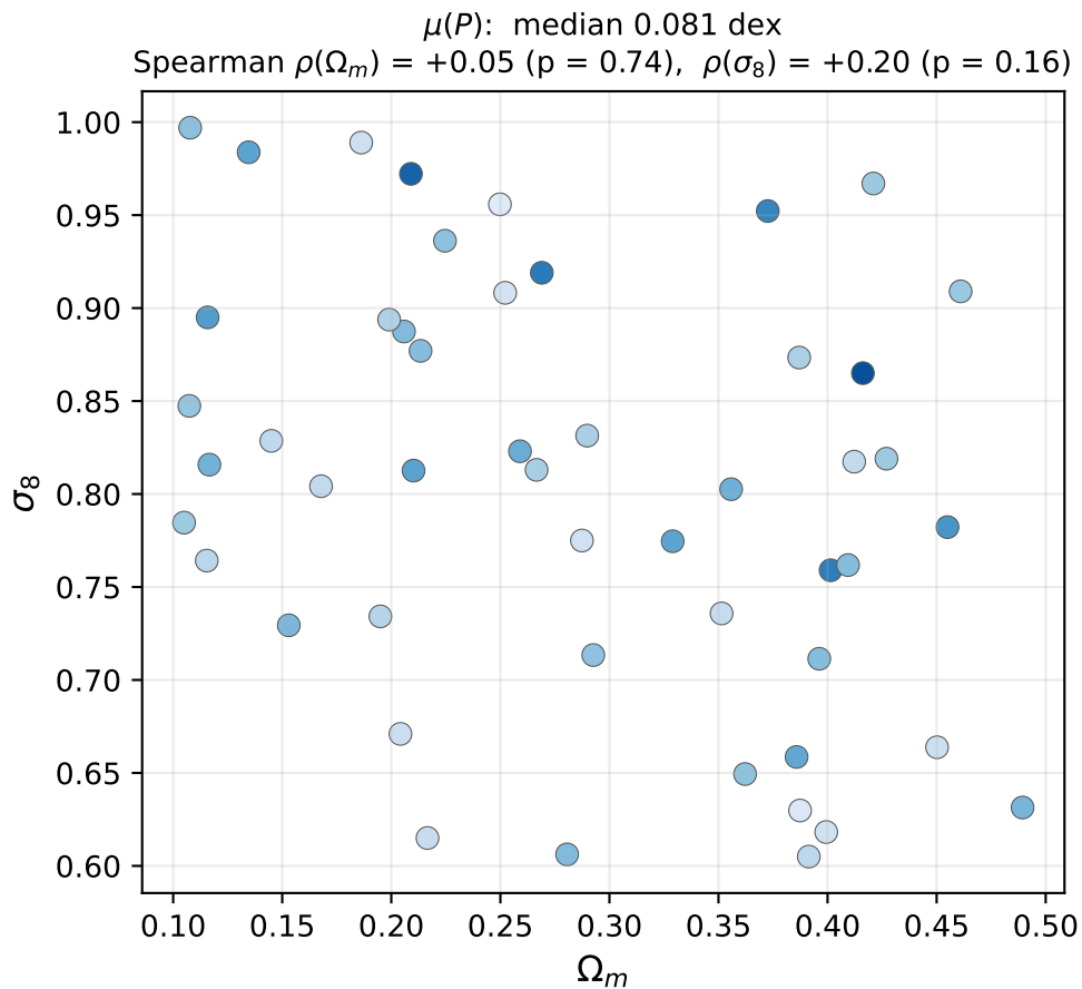
DDPM-2 power-spectrum mismatch across 50 test cosmologies (15 CAMELS maps at each \theta vs 15 generated; lower is better)
