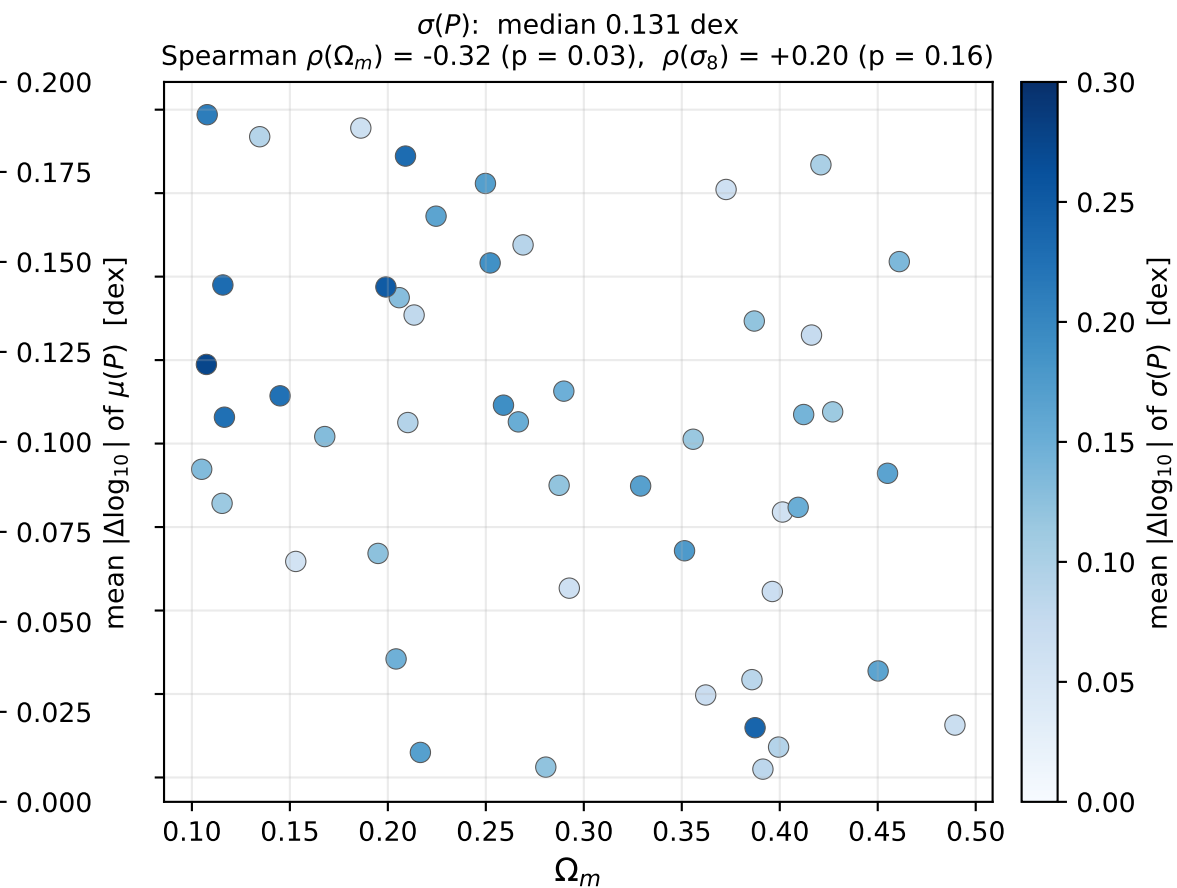
DDPM-2 power-spectrum mismatch across 50 test cosmologies (15 CAMELS maps at each \theta vs 15 generated; lower is better)
