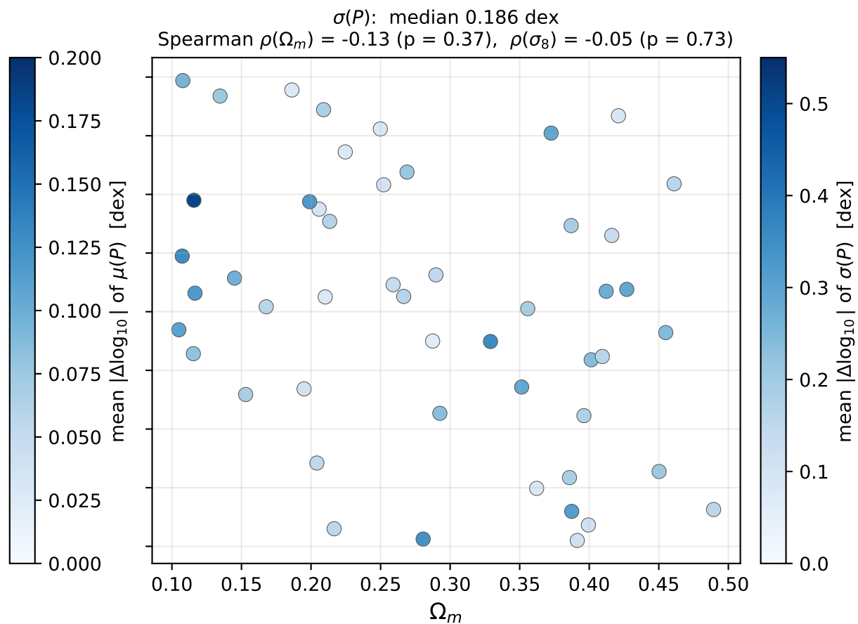
DDPM-6 power-spectrum mismatch across 50 test cosmologies (15 CAMELS maps at each \theta vs 15 generated; lower is better)
