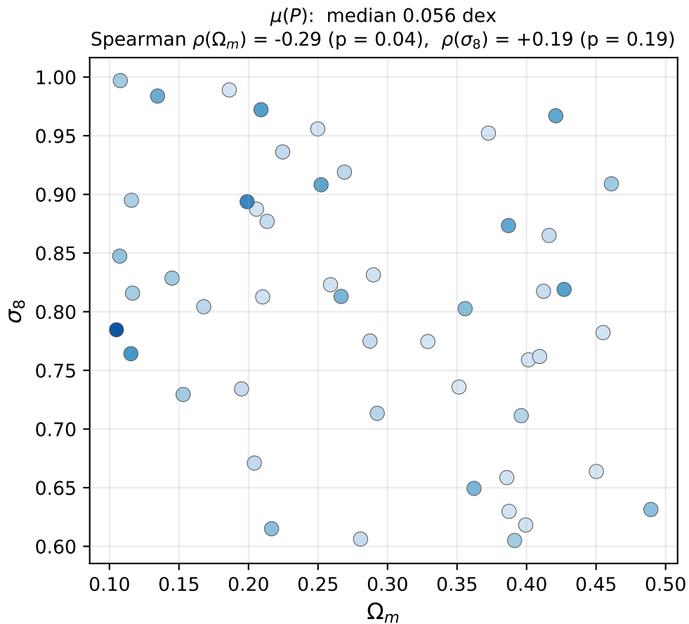
DDPM-6 power-spectrum mismatch across 50 test cosmologies (15 CAMELS maps at each \theta vs 15 generated; lower is better)
