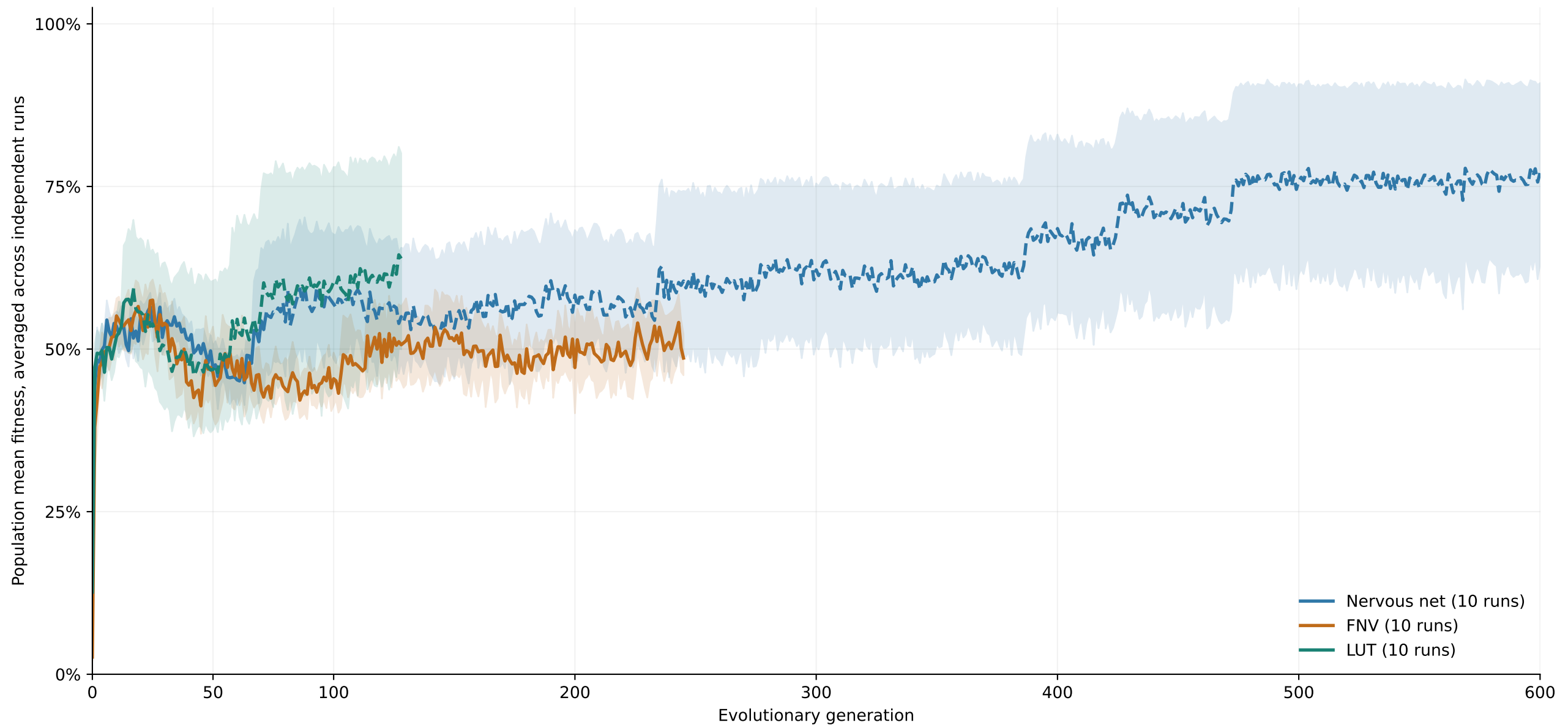
Fig. 14. 2:1 MUX (temporal): developmental evolution through generation 600.
