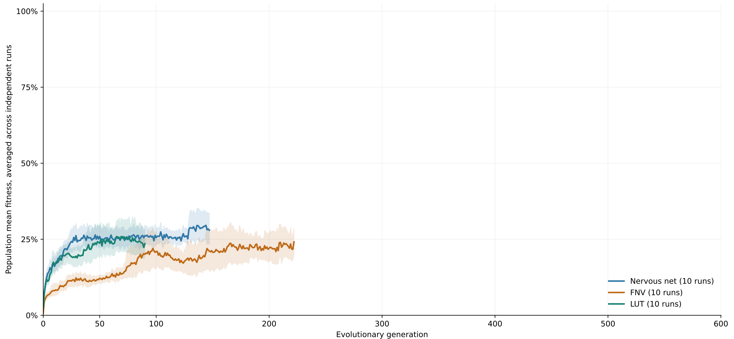
Fig. 12. 2-to-4 decoder (temporal): developmental evolution through generation 600.
